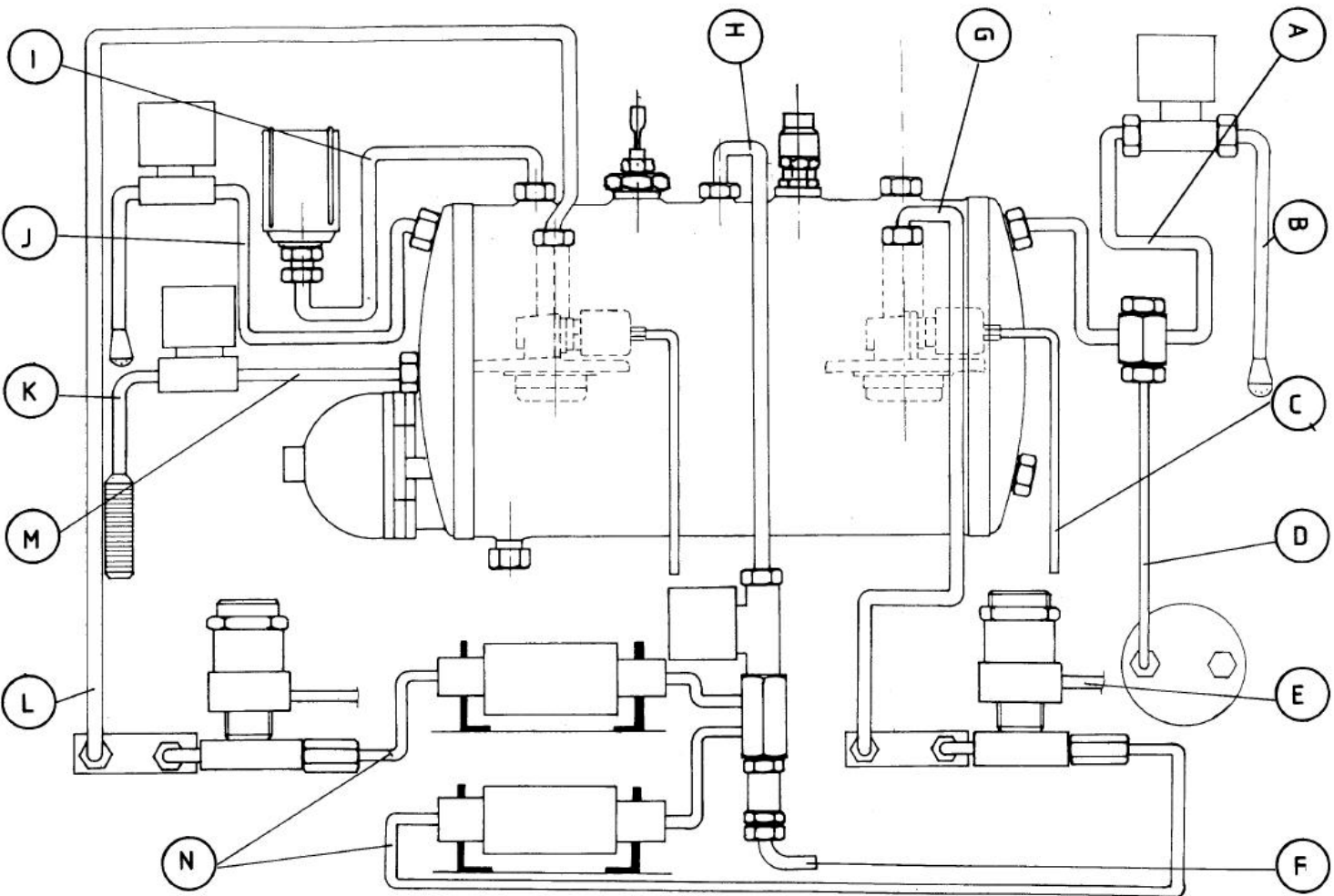
UNIC PHOENIX INTERNAL TUBES
