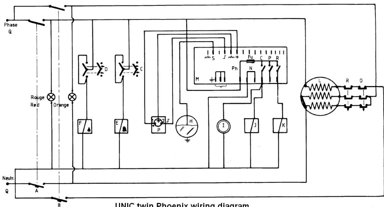
UNIC twin Phoenix wiring diagram
